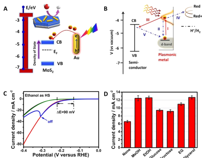
Figure 4. (A) Schematic Au–MoS 2 and energy level diagram illustrating hot electrons injection and change of MoS 2 Fermi level. (B) Different plausible hot electrons transfer pathways likely to occur during SPR. (C) Polarization curves of Au–MoS 2 under 808 nm laser irradiation with (red) or without (black) ethanol as HS. Green line represents the electrochemical behavior of Au–MoS 2 in the dark immediately after one irradiation cycle. Blue line represents the electrochemical behavior upon sudden light-off test. (D) Current density of Au–MoS 2 obtained from i – t curves at –0.23 V under 808 nm laser excitation with a variety of scavenger chemicals. The concentrations of glucose and fructose solutions used were 25 wt %, whereas the rest were 10 vol %.
