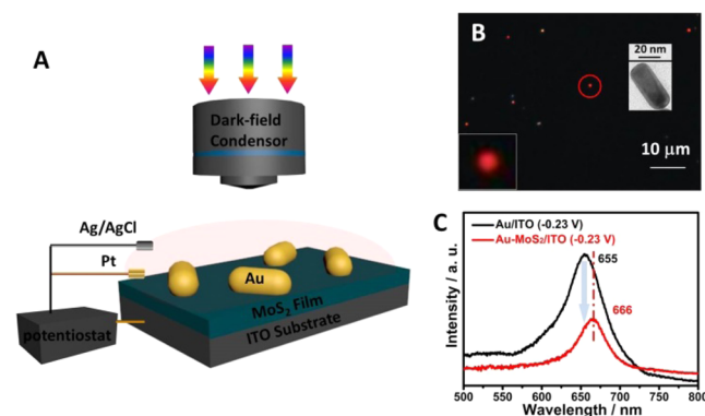
Figure 3. (A) Schematic apparatus for in situ electrochemical SPR scattering measurement in 0.1 M KCl solution under a dark-field microscope. The electrochemical cell consists of a Pt wire as the auxiliary electrode, an Ag/AgCl wire as the reference, and modified indium–tin-oxide (ITO) as the working electrode. (B) Dark-field image of Au rods deposited on ITO in 0.1 M KCl solution, scale bar = 10 \mu\text{m} . Inset shows the dark-field amplified image and TEM image of the labeled Au rods. (C) SPR scattering spectra of Au rods in Au/ITO and Au–MoS 2 /ITO at -0.23 V vs RHE in 0.1 M KCl solution.
